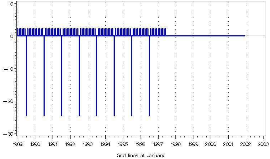
Figure 1: Seasonal Outlier Factor for an Import Series (source: U. S. Census Bureau).
